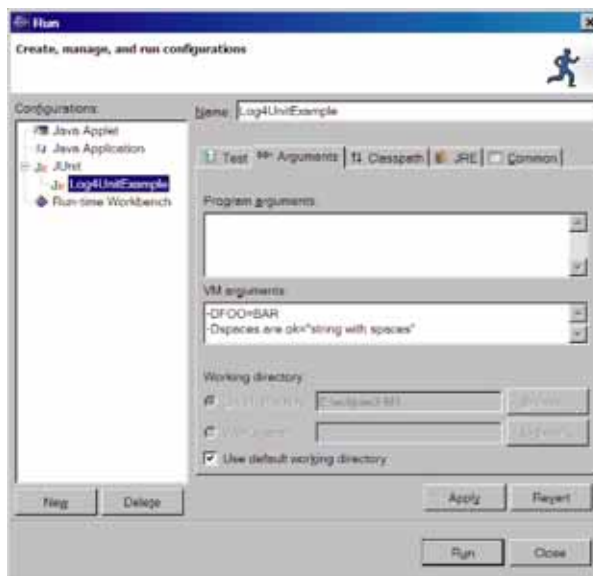
Figure 5.1 Setting system property arguments in Eclipse’s JUnit Run wizard
