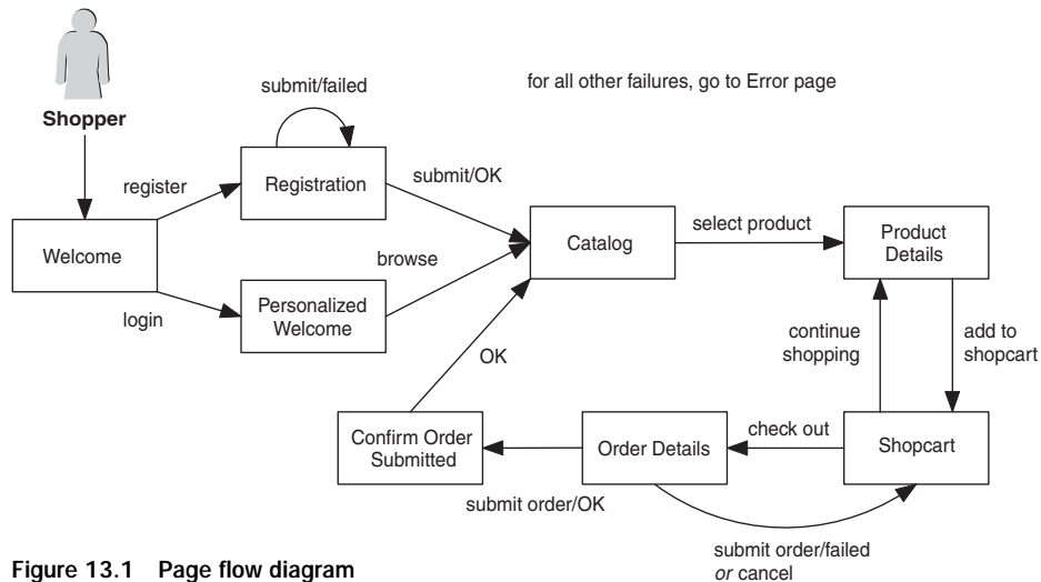
Figure 13.1 Page flow diagram
